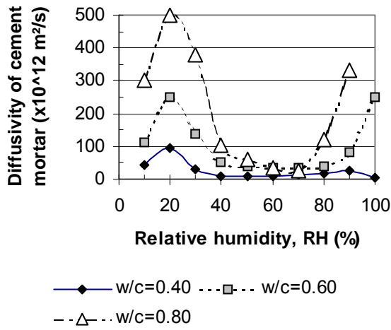
Fig. 9-1: Water diffusivity of cement mortar with different w/c as a function of RH
