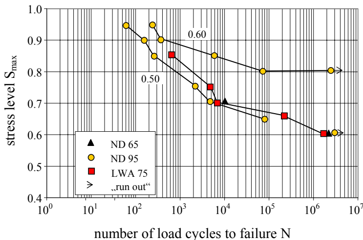
Fig. 7-1: Mean results of ND65, ND95 and LWA75 concrete in fatigue for S_{min}=0.05 and 0.60 , respectively [Petkovic et al. (1990)]
