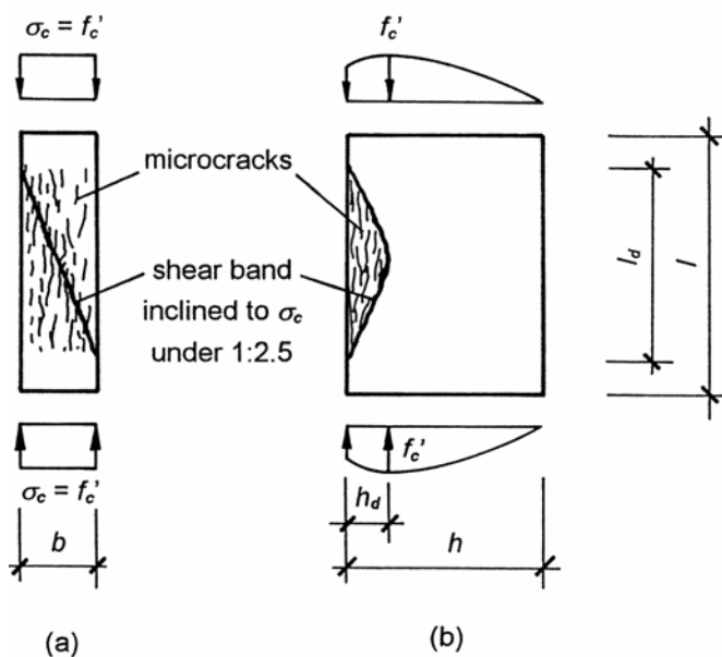
Fig. 4-4: Fracture zone under (a) axial and (b) eccentric compression
