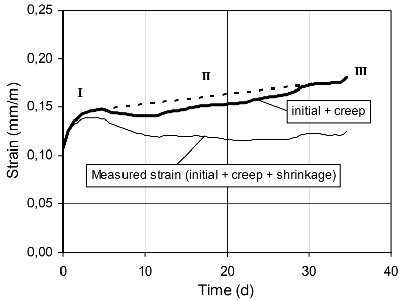
Fig. 6-8: Total strain as function of loading time; concrete C70/85 ( \sigma_{ct} = 4.38 \text{ MPa} , \sigma_{ct} / f_{cm} = 0.90 ); primary (I), secondary (II), and tertiary creep (III) [Rinder (2003)]
